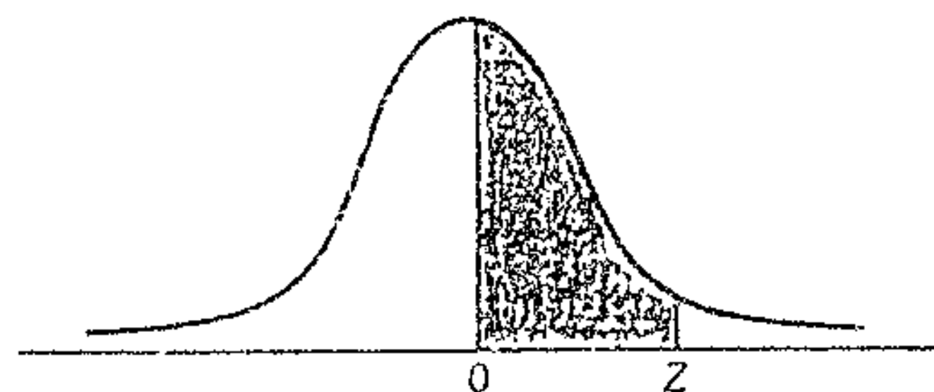
The standardized normal distribution
